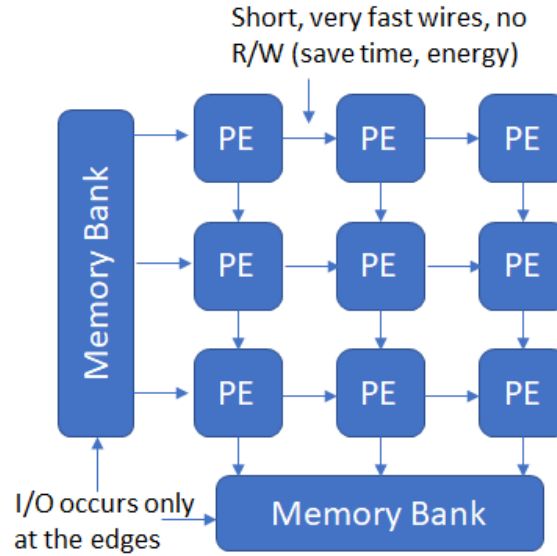
Figure 1: Systolic array operation using Processing Elements
