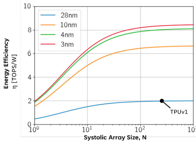
Figure 2: Energy efficiency limitation of leading semiconductor technology nodes
