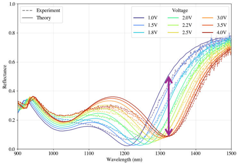
Figure 11: Spectral reflectivity of the metasurface; solid lines represent simulated responses and dotted lines are experimental data. As shown by the purple arrow, at a given wavelength, changing the metasurface pixel's voltage modifies its reflectivity, enabling optical multiplication
